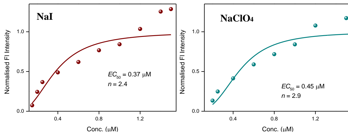
Figure S21. Determination of EC_{50} values from concentration-dependent plots for I - and ClO 4 - from Figure S20 for polymer 1a .
